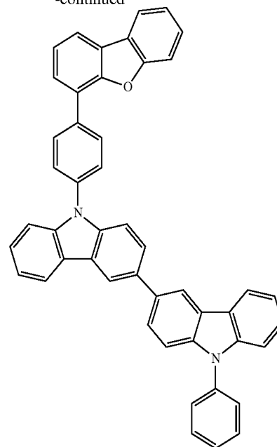
Compound 3H
