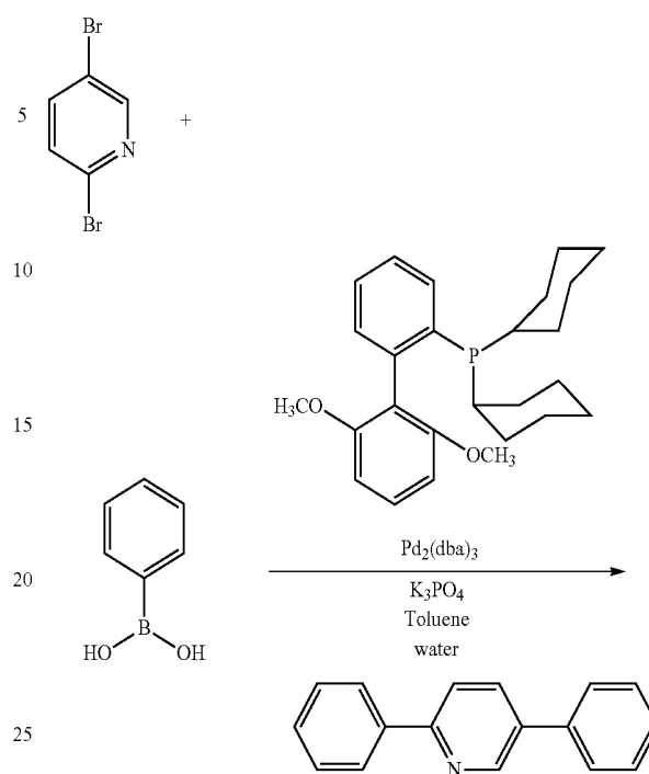
Synthesis of 2, 5-diphenylpyridine
